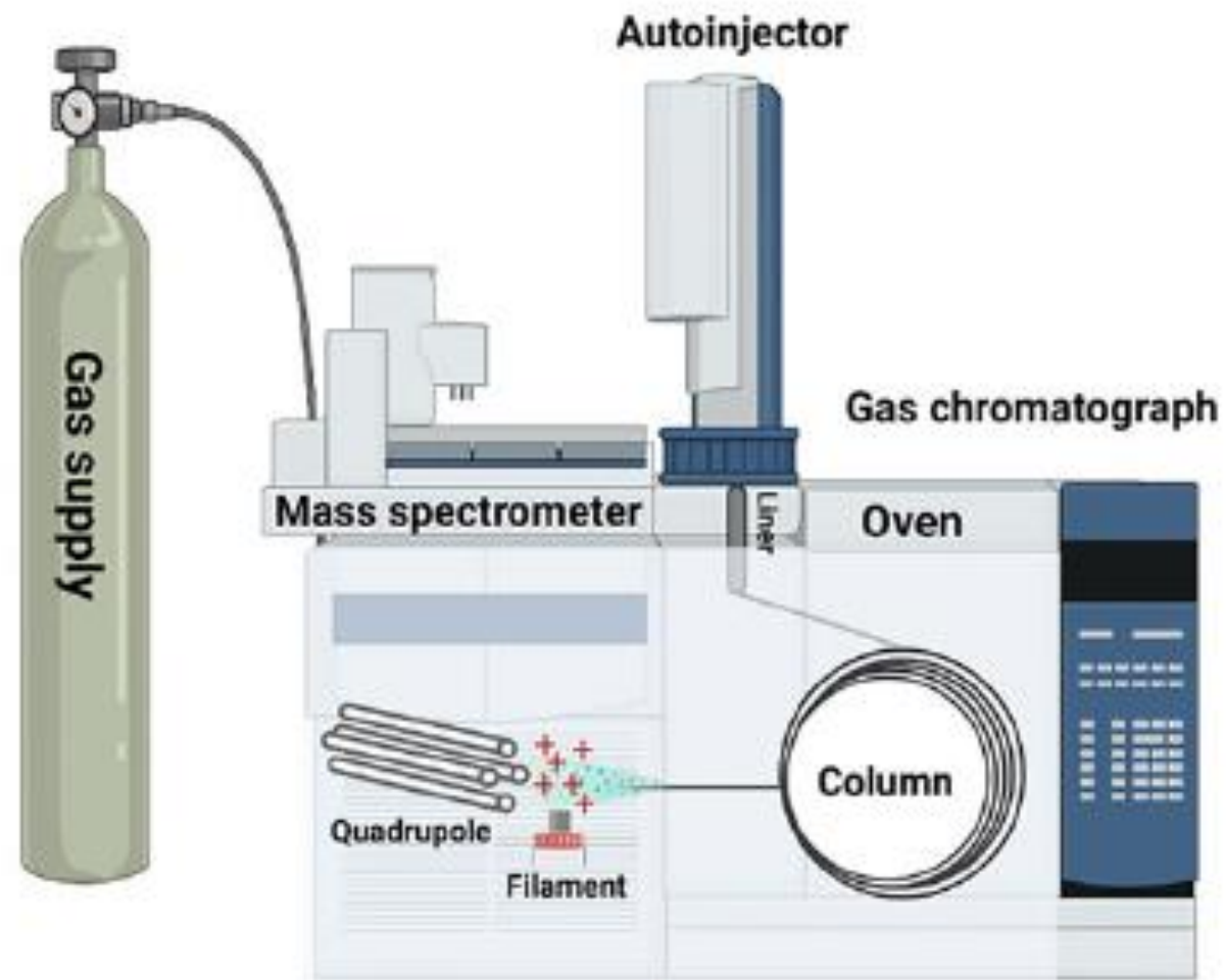
Fig. 1.3 The basic components of a GC-MS system (figure made with biorender.com )
