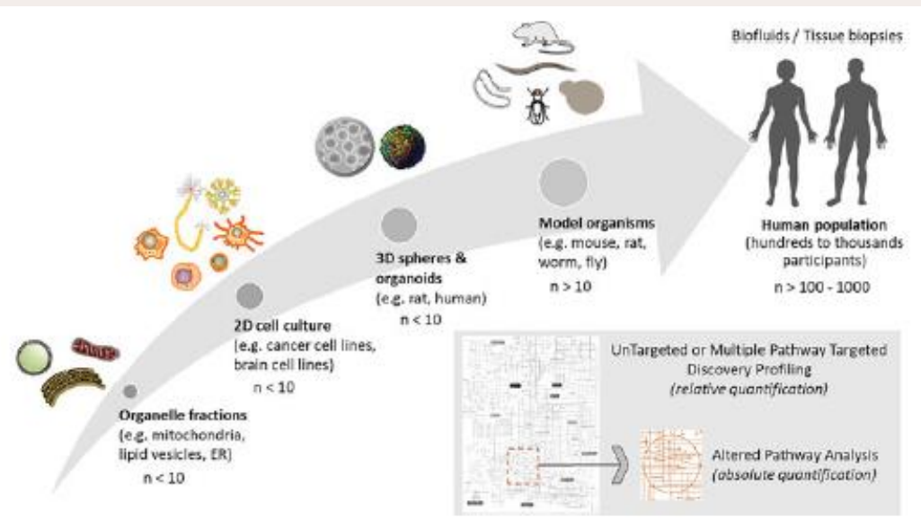
Fig. 1.12 From model systems to human population studies. Due to its high-throughput and phenotyping capacity, different metabolomics and lipidomics approaches, from untargeted screening to targeted quantification, can be applied from different model systems, demanding low numbers of independent biological replicates, to clinical research studies, demanding high numbers of participants due to high human inter-individual variability. An estimated number of replicates is indicated below each studied system. It is mandatory to validate the results of untargeted profiling by targeted quantification, particularly in human population studies, and also to allow for data cross-comparability. The figure was reproduced from [39]
