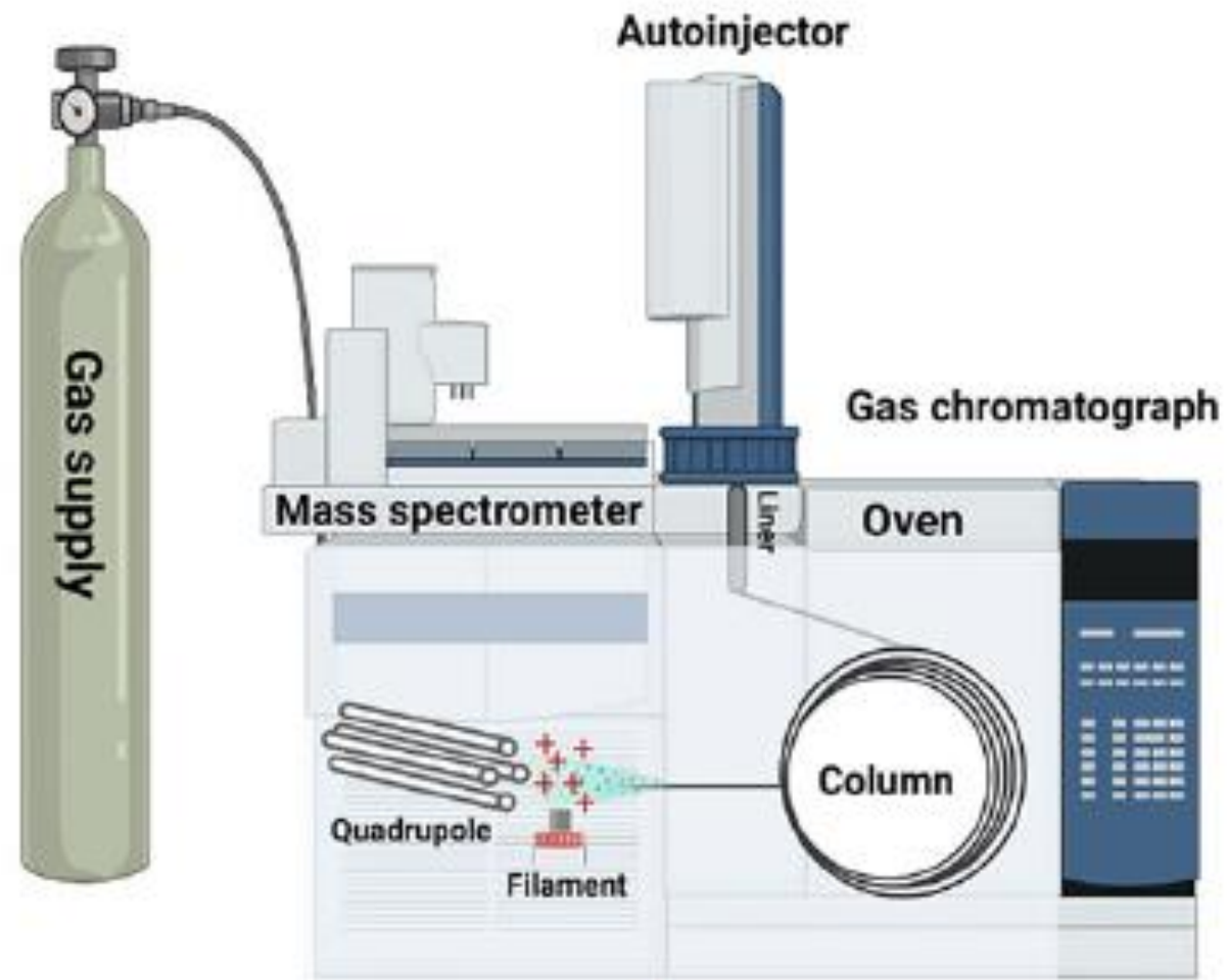
Fig. 1.3 The basic components of a GC-MS system (figure made with biorender.com )
